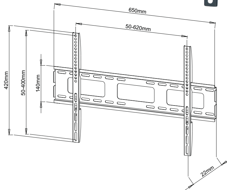
(Schematic Diagram)
